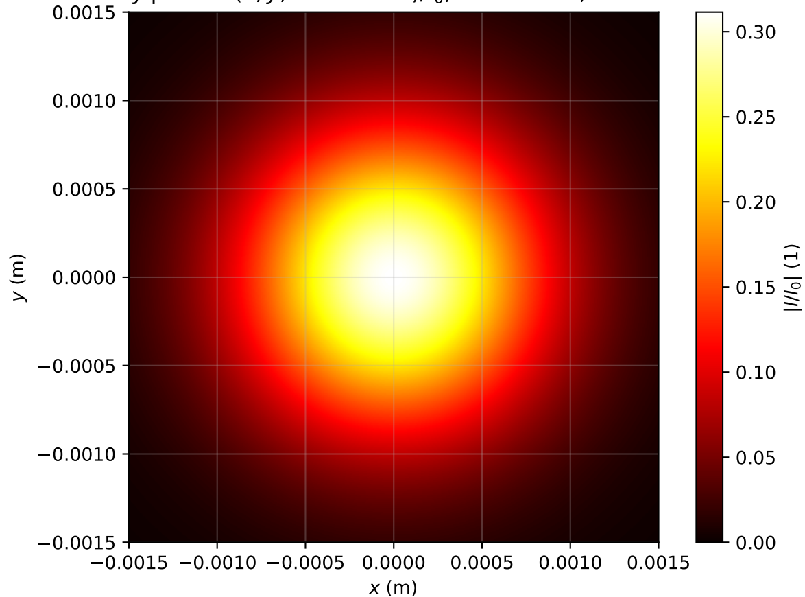
Intensity profile I(x, y, z = 3.742m)/I_0 , P_{in}=0.3P_{cr} , artificial time
